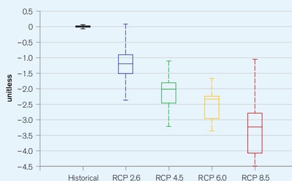
FIGURE 11. Annual SPEI Drought Index in Egypt for the period, 1986 to 2099 51
