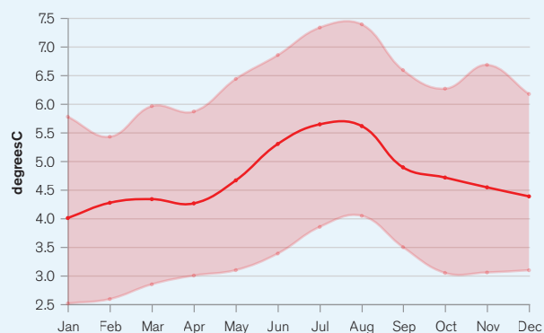
FIGURE 10. Average daily max temperature for Egypt 44
