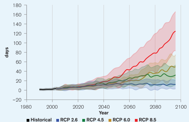
FIGURE 14. Warm Spell Duration Index in Egypt for the period 1986 to 2099 58
