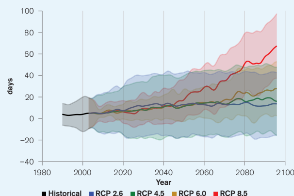
FIGURE 15. Days with a Heat Index >35°C 65
