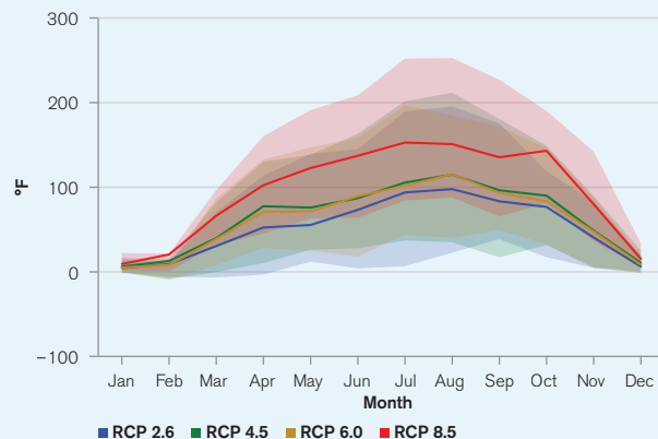
FIGURE 13. Change in Cooling Degree Days (65°F) in Egypt for the period 2040–2059 57
