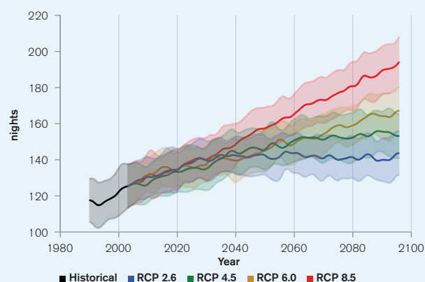
FIGURE 16. Number of Tropical Nights (Tmin >20°C) 66
