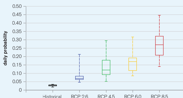
FIGURE 9. Projected change in the probability of observing a heat wave in Nepal by 2080–2099. A 'Heat Wave' is defined as a period of 3 or more days where the daily temperature is above the long-term 95th percentile of daily mean temperature. 19
