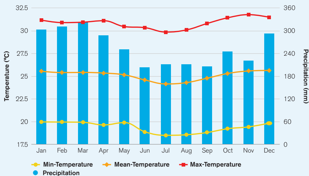
FIGURE 2. Average monthly mean, max, and min temperatures and rainfall in PNG (1991–2020) 17
