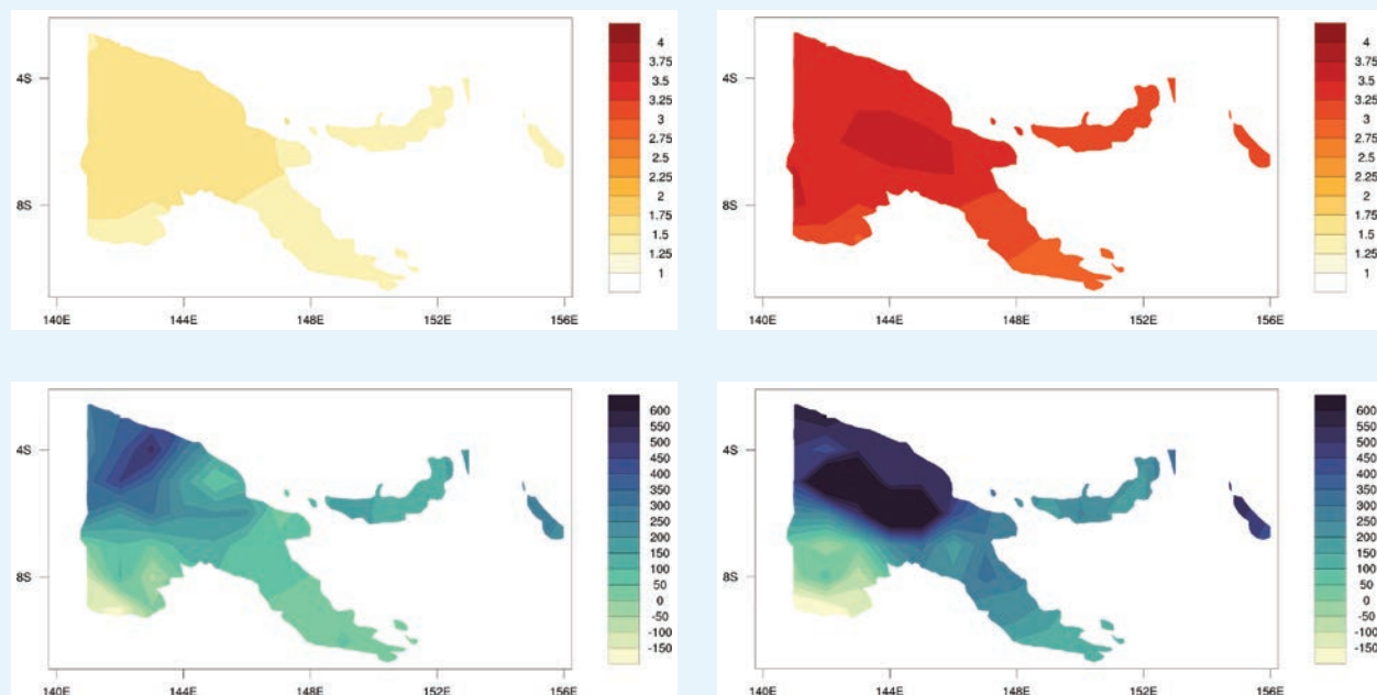
FIGURE 5. CMIP5 ensemble projected change (32 GCMs) in annual temperature (top) and precipitation (bottom) by 2040–2059 (left) and by 2080–2090 (right) relative to 1986–2005 baseline under RCP8.5 26
