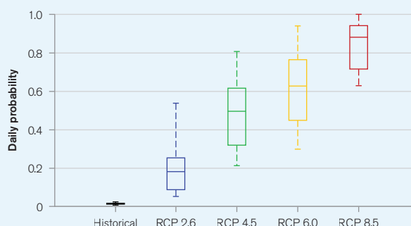
FIGURE 9. Projected change in the probability of observing a heat wave in PNG for the period 2080–2099. A 'Heat Wave' is defined as a period of 3 or more days where the daily temperature is above the long-term 95th percentile of daily mean temperature. 26
