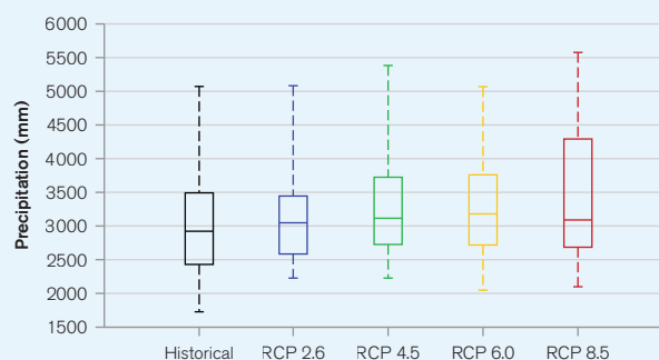
FIGURE 8. Boxplots showing the projected average annual precipitation for PNG in the period 2080–2099 26
