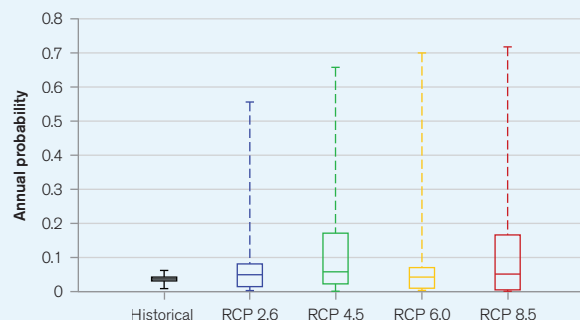
FIGURE 10. Boxplots showing the annual probability of experiencing a ‘severe drought’ in PNG (−2 SPEI Index) in 2080–2099 under four emissions pathways 26
