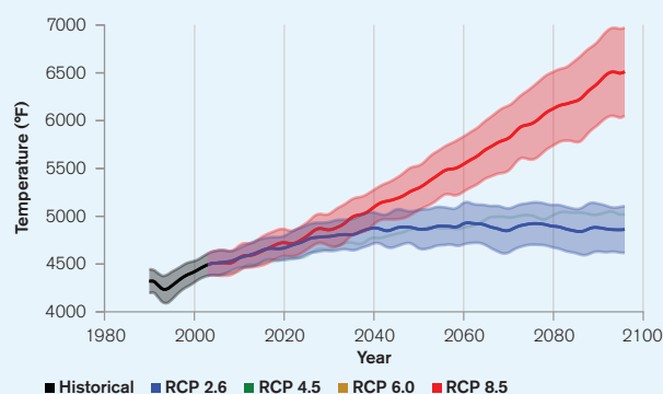
FIGURE 12. Historic and projected annual cooling degree days in PNG (cumulative degrees above 65°F) under RCP2.6 (blue) and RCP8.5 (red). The values shown represent the median of the multi-model ensemble with the shaded areas showing the 10–90th percentiles. 26
