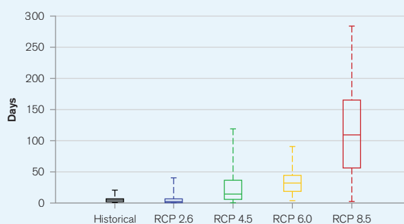
FIGURE 13. Historical (1986–2005) and projected (2080–2099) annual count of days with Heat Index >35°C under four emissions pathways in PNG 26
