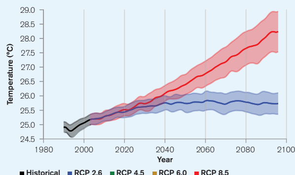
FIGURE 6. Historic and projected average annual temperature in PNG under RCP2.6 (blue) and RCP8.5 (red) estimated by the CCKP model ensemble. Shading represents the standard deviation of the model ensemble. 27
