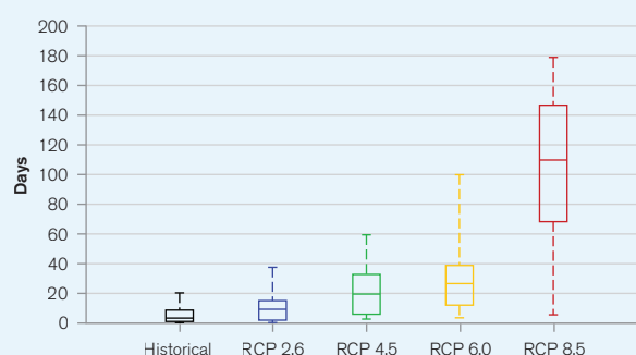
FIGURE 11. Ensemble estimate of the annual number of very hot ( T_{max} > 35^{\circ}\text{C} ) days in 2080–2099 under four emissions pathways in PNG 26
