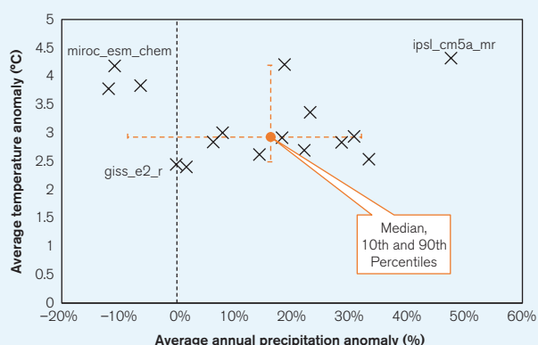
FIGURE 4. 'Projected average temperature anomaly' and 'projected annual rainfall anomaly' in PNG. Outputs of 16 models within the ensemble simulating RCP8.5 over the period 2080–2099. Models shown represent the subset of models within the ensemble which provide projections across all RCPs and therefore are most robust for comparison. 25 Three models are labelled.
