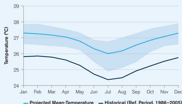
FIGURE 7. Projected monthly temperature, in relation to the Historical Reference Period, 1986–2005, for PNG for the period 2040–2059 under RCP8.5. The value shown represents the median of the model ensemble with the shaded areas showing the 10th–90th percentiles. 26
