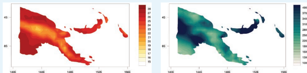
FIGURE 3. Annual mean temperature (°C) (left), and annual mean rainfall (mm) (right) in PNG over the period 1991–2020 18
